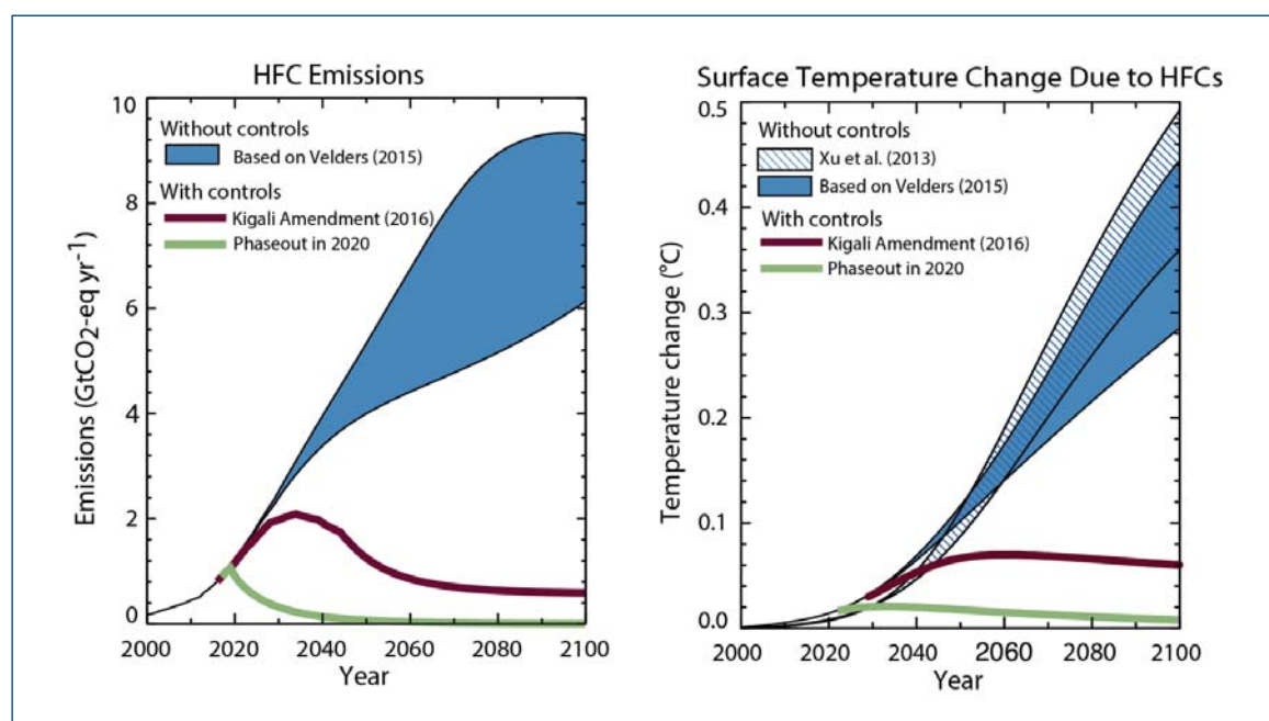
The contribution of HFCs to man-made climate change in different scenarios.
