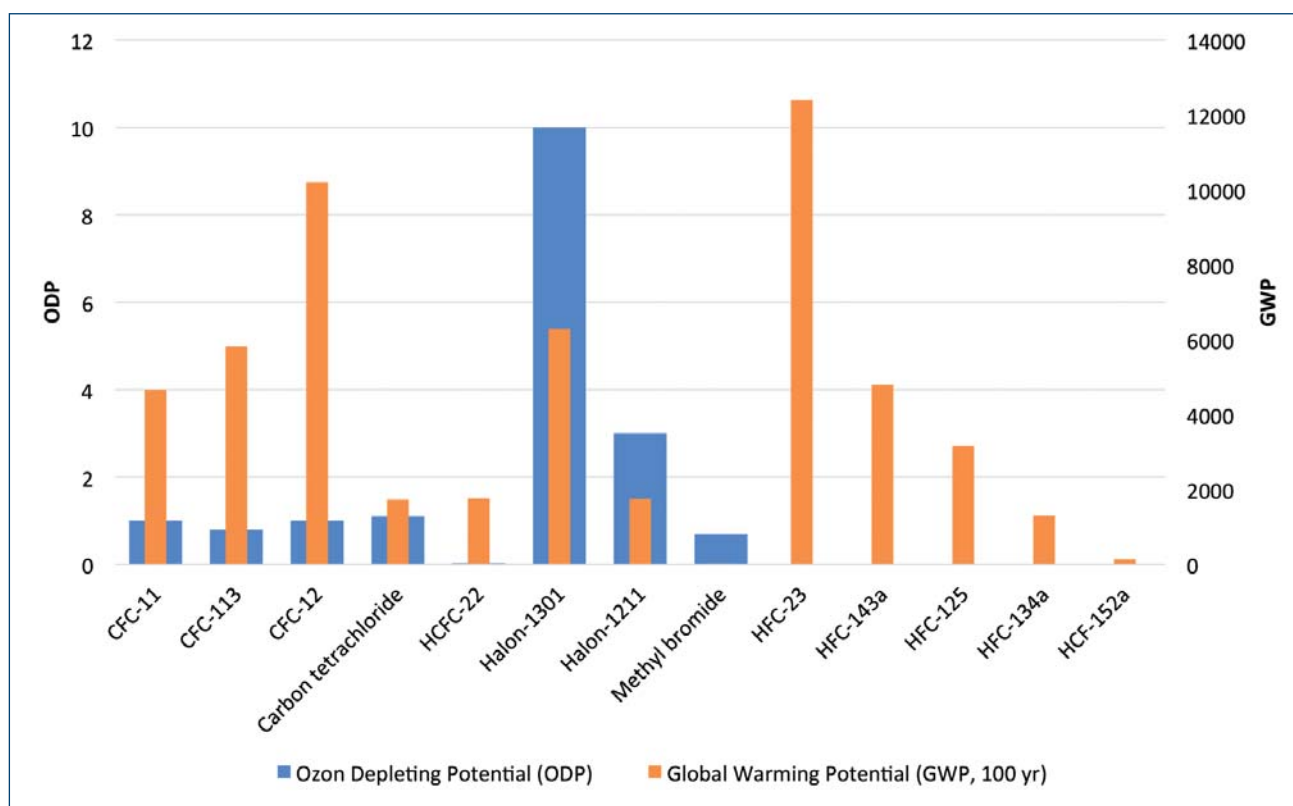
Comparing the Ozone Depleting Potentials (ODPs) and Global Warming Potentials of the main products covered by the Montreal Protocol.
