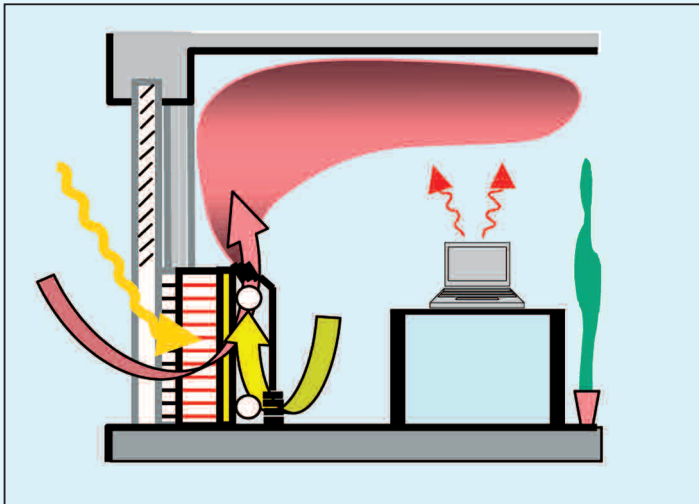
Figure 7. On a sunny winter day mixed convection is the adequate ventilation method.
