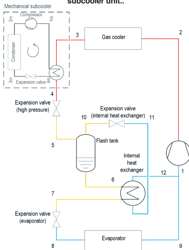
Figure 3. Standard R744 booster cycle with mechanical subcooler unit..
