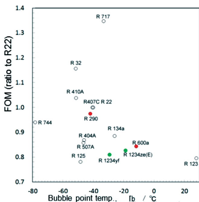
(a) In case of small pressure losses in heat exchangers and connecting pipes
