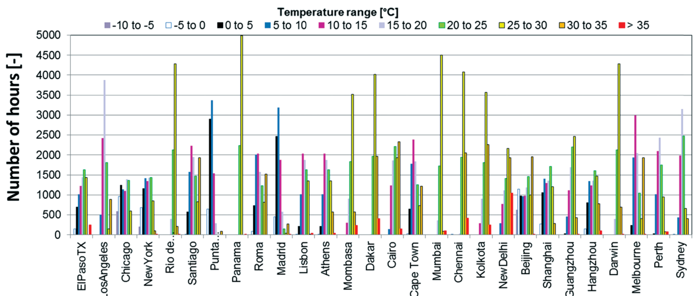
Figure 1. Temperature bins for selected cities. (Source Meteonorm)
