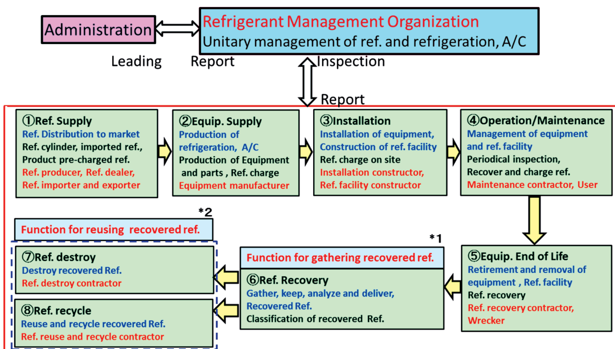
Figure 4. Refrigerant distribution flow (yellow arrow) and proposed management system by JSRAE
