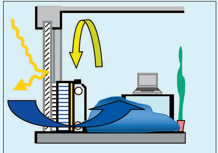
Figure 8. On a sunny summer day displacement ventilation is applied.
