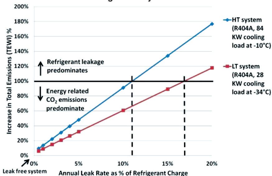
Figure 4. Impact of refrigerant leakage on TEWI for typical R404A refrigeration systems 7
