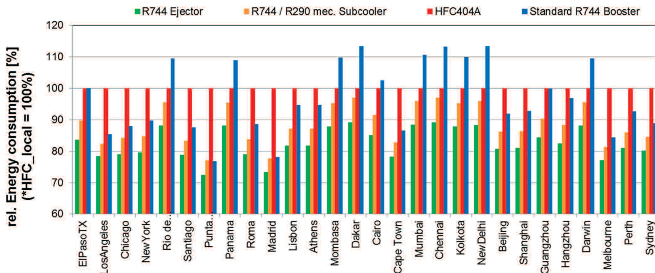
Figure 8. Relative annual energy consumption of alternative commercial refrigeration systems. Local HFC systems are set to 100%.
